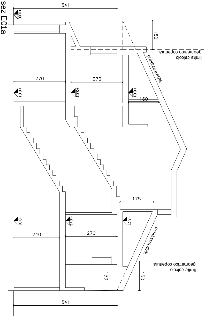
PIANO TERRA
